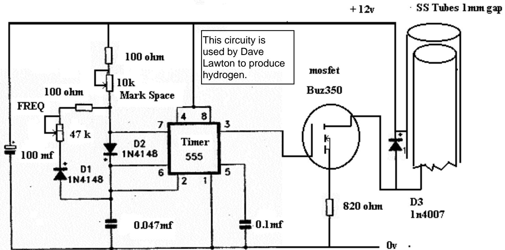
TEST SETUP Dave Lawton
